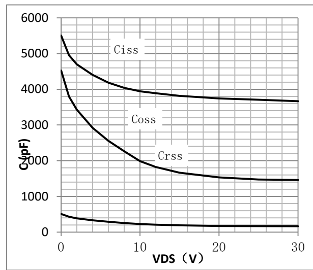
Fig.2 Capacitance Characteristics
